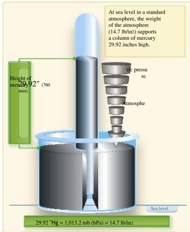
Figure 11-6. Mercurial barometer.
