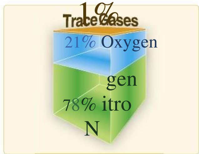
Figure 11-1. Composition of the atmosphere.
