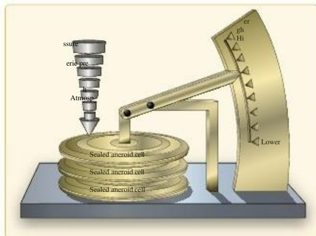
Figure 11-7. Aneroid barometer.
